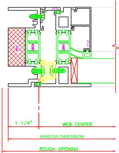
421 JAMB 325 PROJECT OUT \ FIXED 4-BAR ARMS
